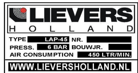
Fig. 1: Ratingplate LAP 45
