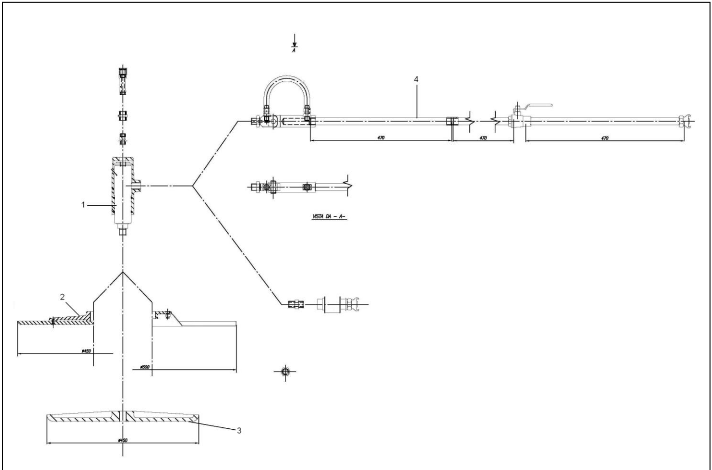
Fig. 2: Parts pneumatic power trowel LAP 45
