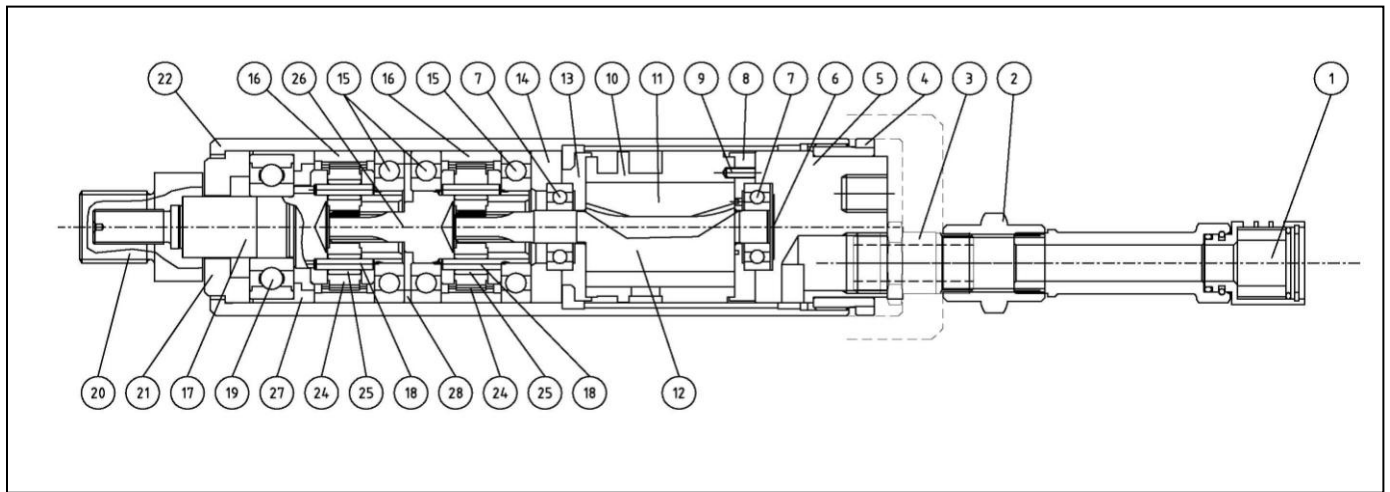
Fig. 3: Parts pneumatic motor LAP 45
