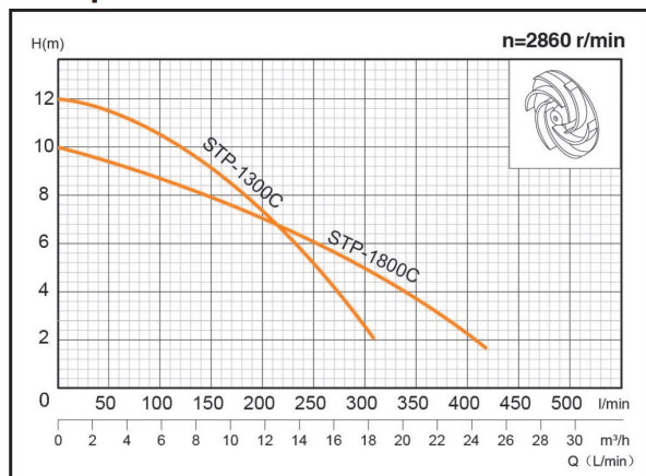
Pumpekurve 1300C
